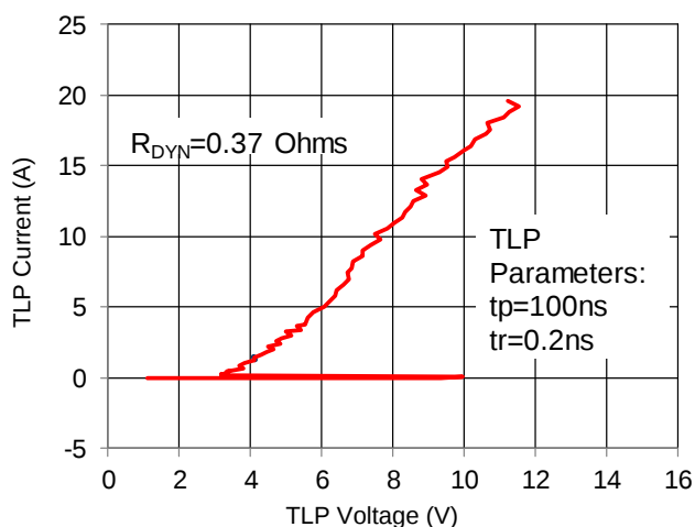
Figure 3: TLP Positive I-V Curve
