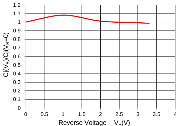
Figure 6: Normalized Junction Capacitance vs. Reverse Voltage
