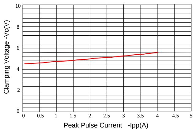
Figure 5: Clamping Voltage vs. Peak Pulse Current
